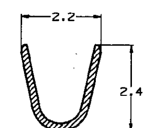
SECT. B-B
