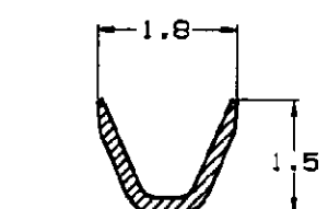
SECT. A-A
