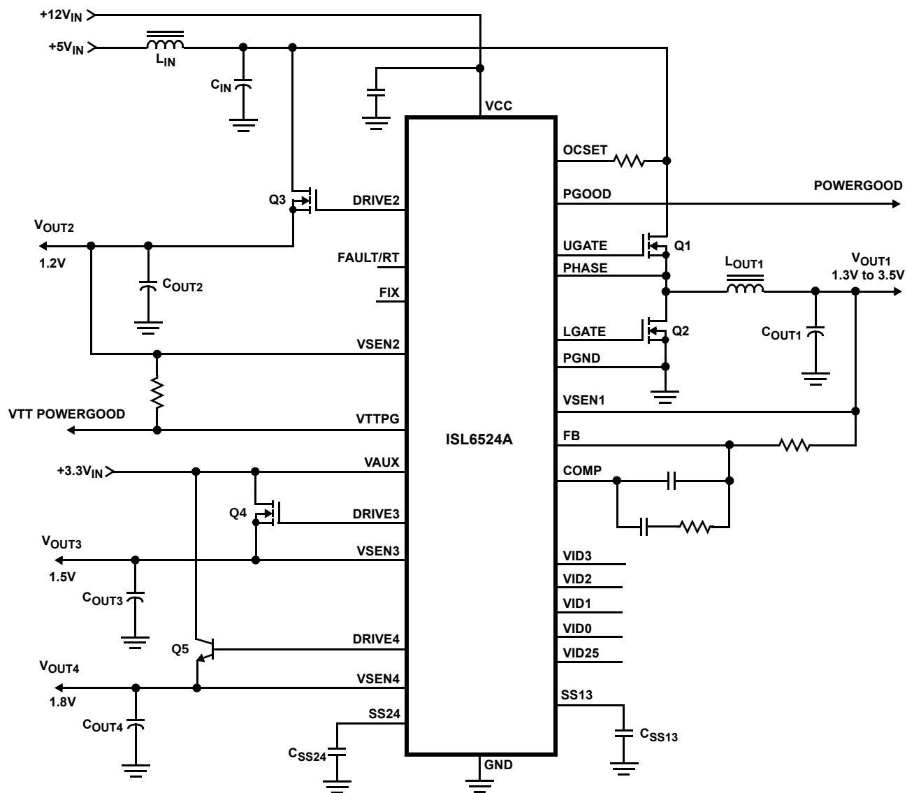
FIGURE 3. TYPICAL APPLICATION
