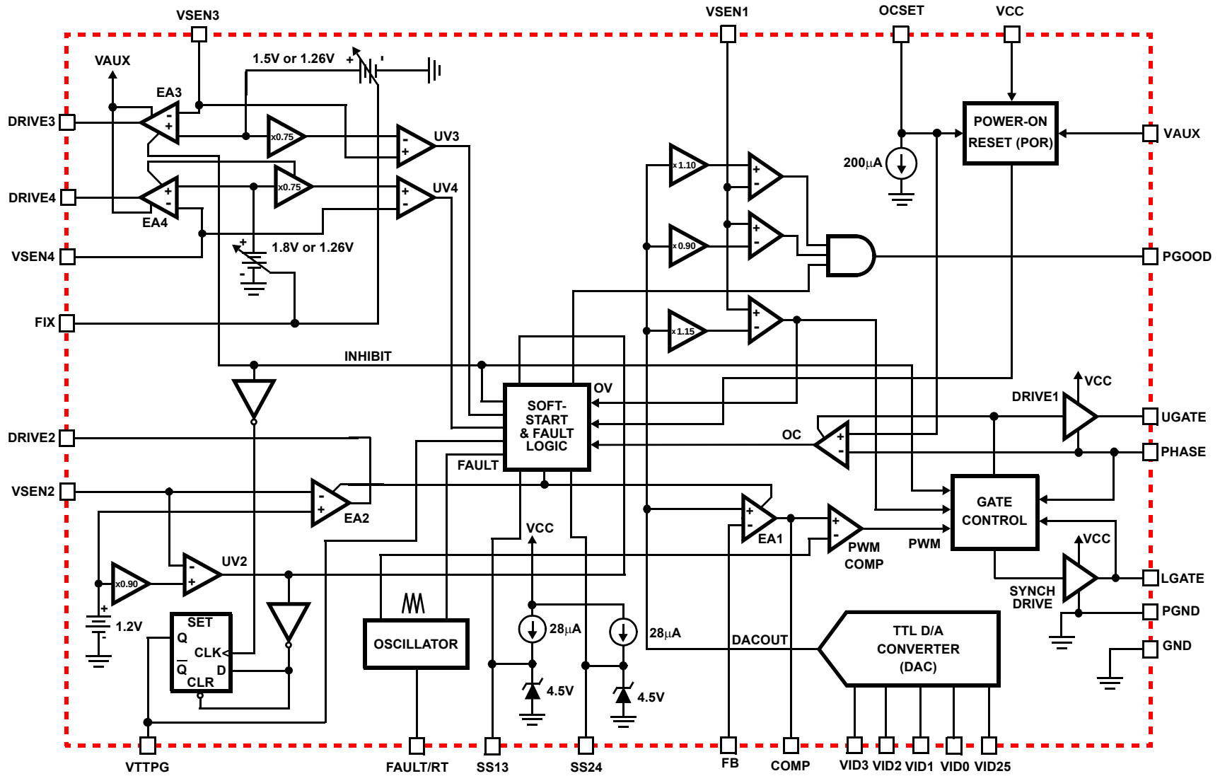
FIGURE 1. BLOCK DIAGRAM
