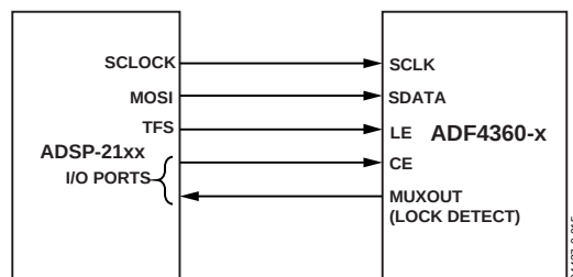
Figure 18. ADSP-21xx to ADF4360-x Interface
