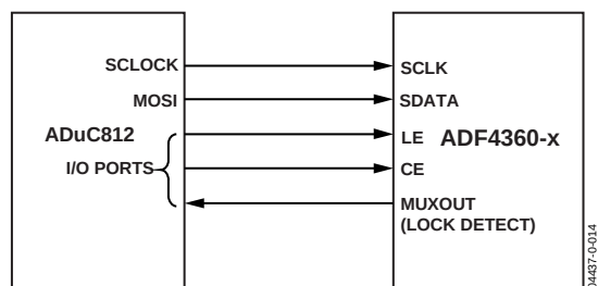
Figure 17. ADuC812 to ADF4360-x Interface
