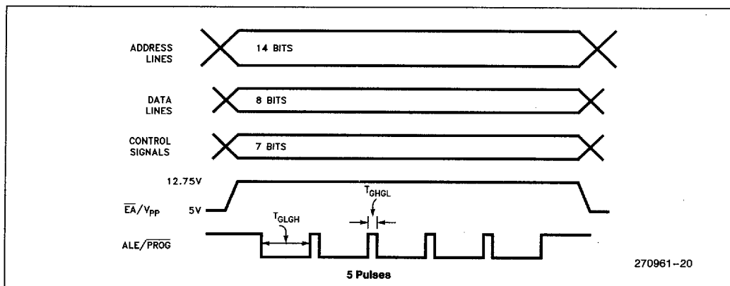
Figure 12. Programming Signal's Waveforms
