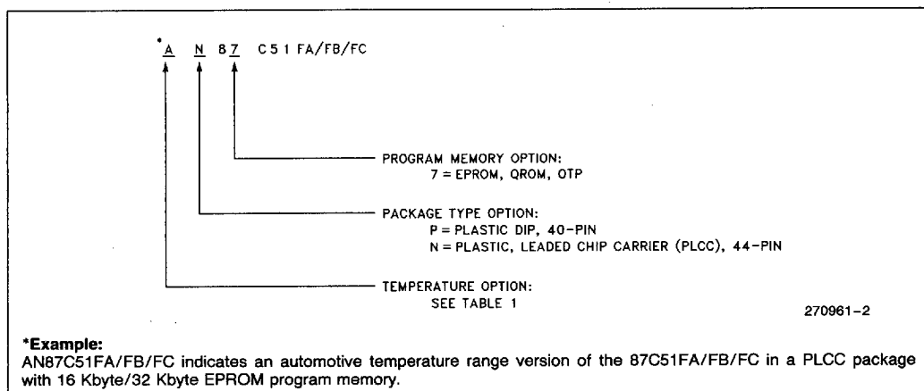
Figure 2. Package Options
