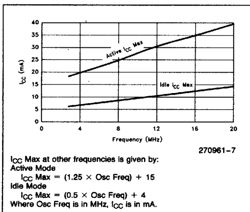
Figure 6. I_{CC} vs Frequency
