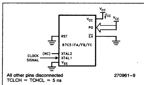
Figure 8. I_{CC} Test Condition Idle Mode
