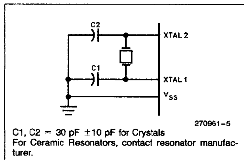
Figure 4. Oscillator Connections
