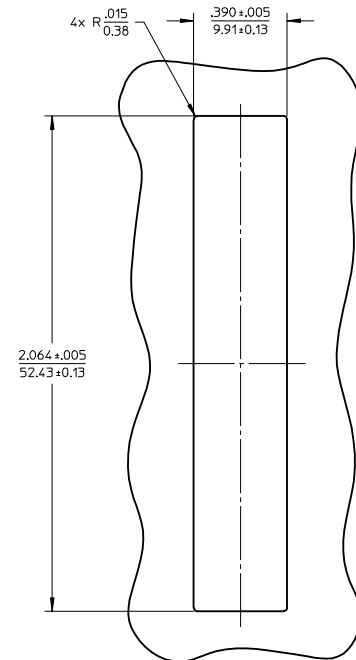
RECOMMENDED MOUNTING PATTERN
