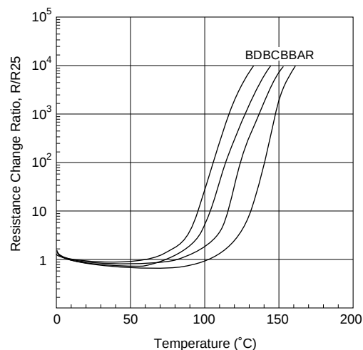
[Resistance-Temperature Characteristic]
