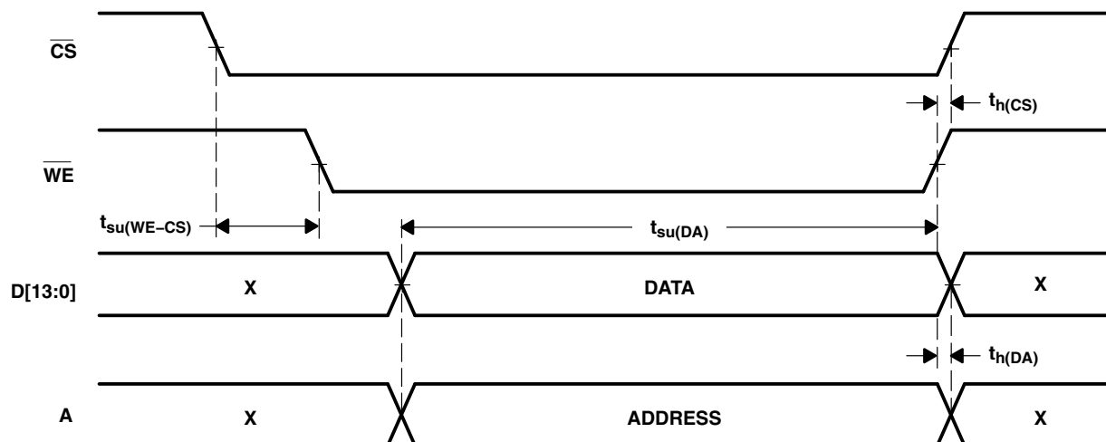
Figure 3. Write Timing
