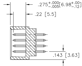
SECTION X-X
