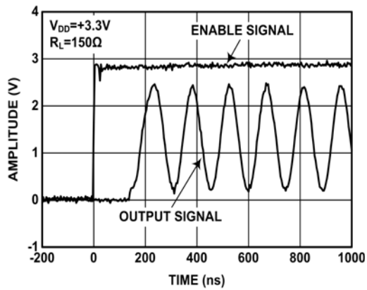
FIGURE 15. ENABLE TIME
