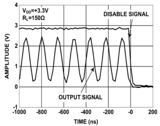
FIGURE 16. DISABLE TIME
