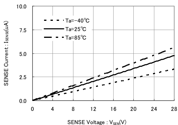
XC6408E ( V_{DF}=11.0V )
