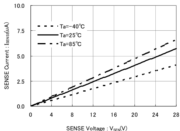
XC6408E ( V_{DF}=16.0V )
