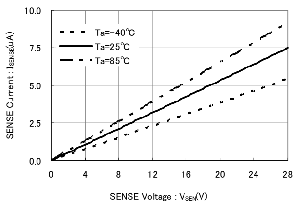
XC6408E ( V_{DF}=2.0V )
