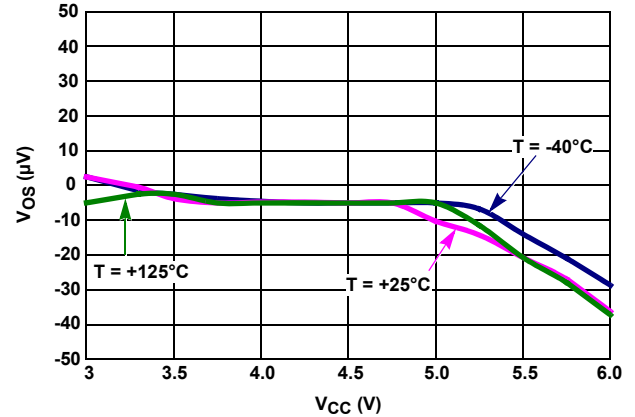
FIGURE 28. AUXILIARY V_{SHUNT} V_{OS} vs V_{CC}
