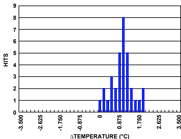
FIGURE 51. INTERNAL TEMPERATURE ACCURACY AT T = -40^\circ\text{C}
