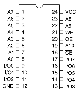
PDIP, SOIC Top View
