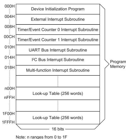
Program Memory
