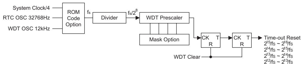
Watchdog Timer
