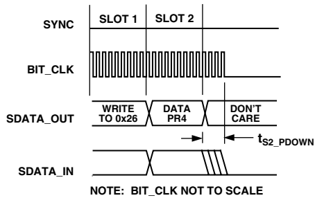
Figure 6. AC-Link Low Power Mode Timing
