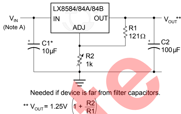
Figure 5 – 1.2V – 8V Adjustable Regulator
