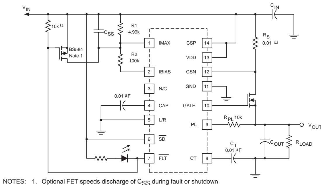
Figure 5. Application Circuit
