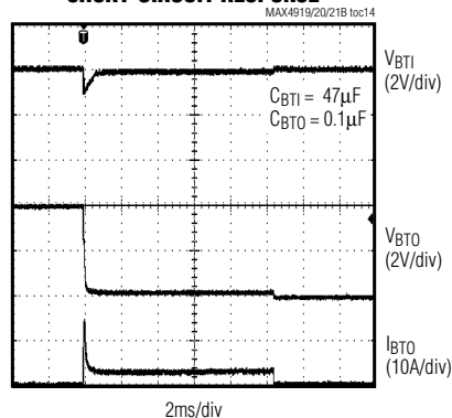
SHORT-CIRCUIT RESPONSE
