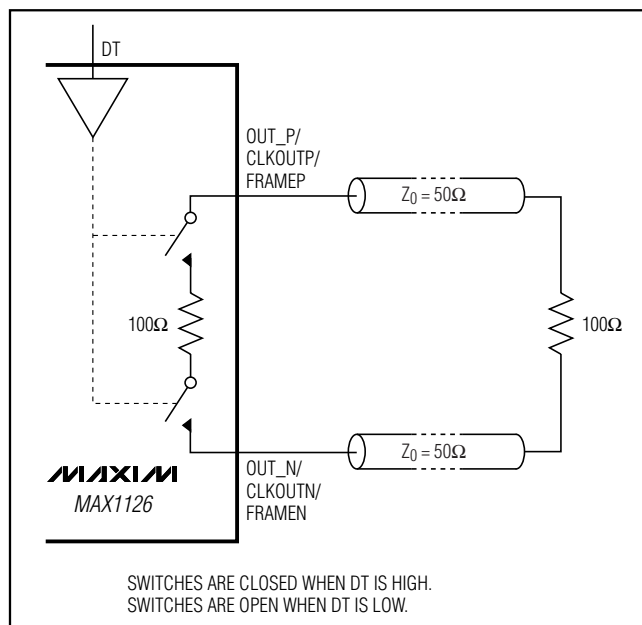
Figure 8. Double Termination
