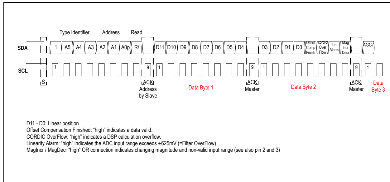
Figure 9. I 2 C Read Out by an \mu C-Master
