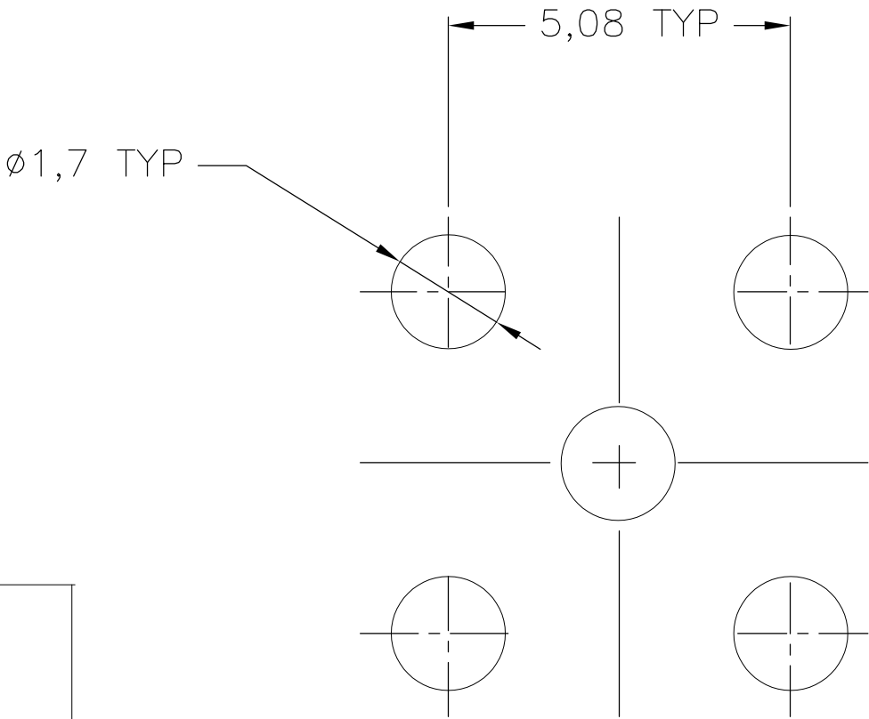
RECOMMENDED MOUNTING HOLE
