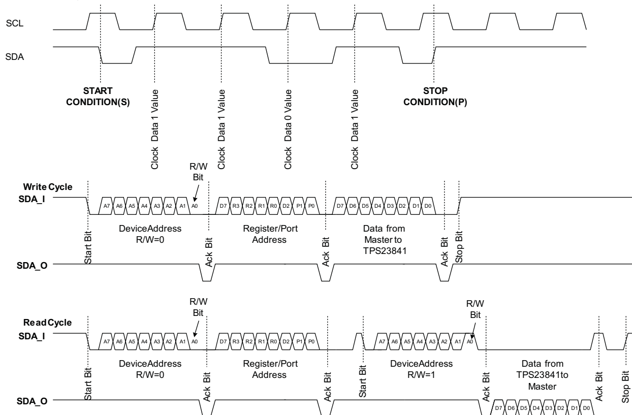
Figure 16. I 2 C Read/Write Cycles
