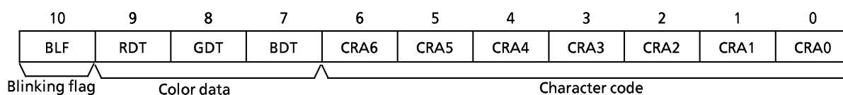
Figure 3-10. Bit Configuration of Display Memory
