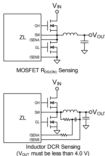
FIGURE 16. Current Sensing Methods
