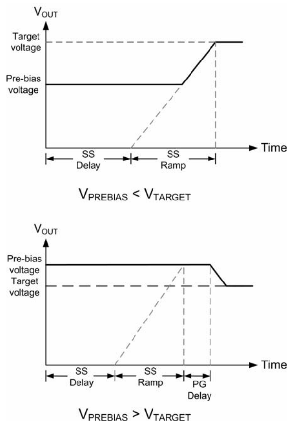
FIGURE 19. Output Responses to Pre-bias Voltages
