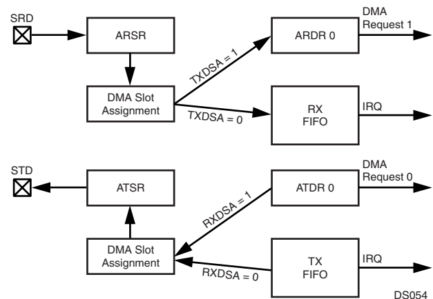
Figure 57. IRQ/DMA Support in Normal Mode
