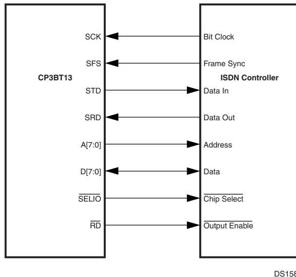
Figure 65. CP3BT13/ISDN Controller Connections
