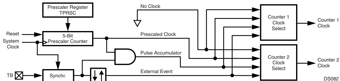
Figure 89. Multi-Function Timer Clock Source
