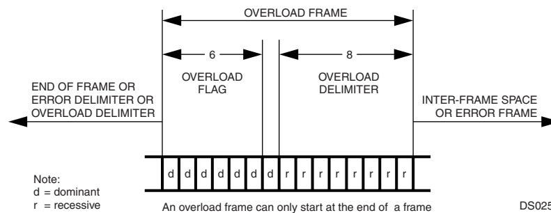
Figure 32. Overload Frame
