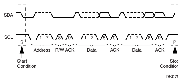
Figure 86. A Complete ACCESS.bus Data Transaction
