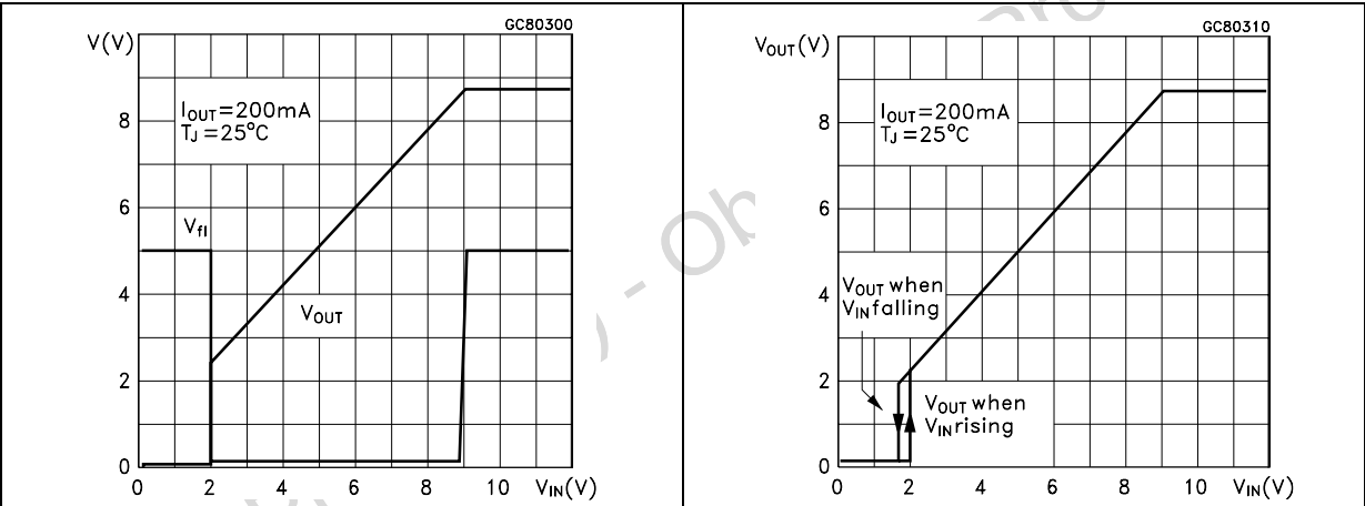
Figure 7. Output and flag voltage vs inp. volt. Figure 8. Output voltage vs input voltage
