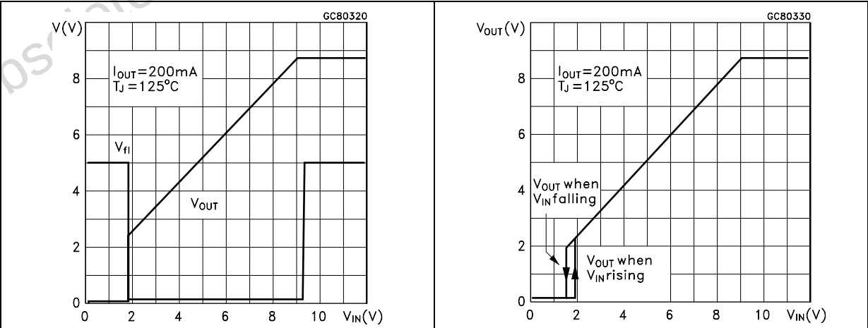
Figure 7. Output and flag voltage vs inp. volt. Figure 8. Output voltage vs input voltage
