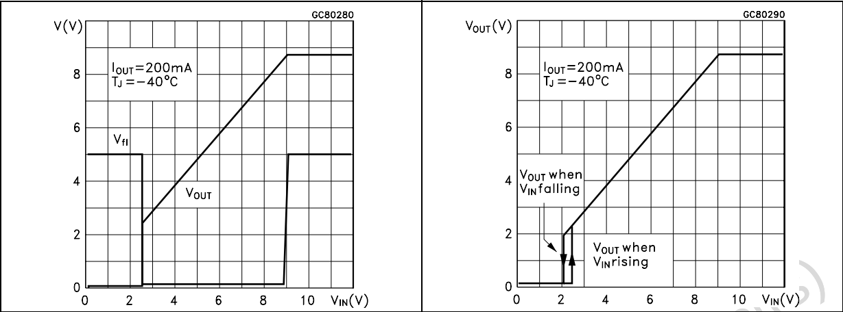
Figure 5. Output and flag voltage vs input voltage Figure 6. Output voltage vs input voltage
