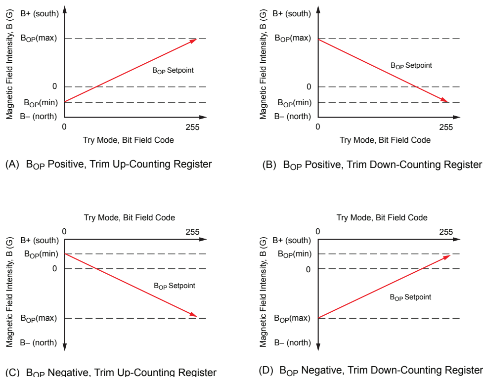
Figure 14. B OP profiles for each of the four B OP Selection virtual registers available in Try mode.
