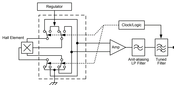
Figure 5. Concept of Chopper Stabilization Technique
