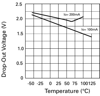
Drop-Out Voltage v Temperature
