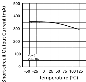
Peak Output Current v Temperature
