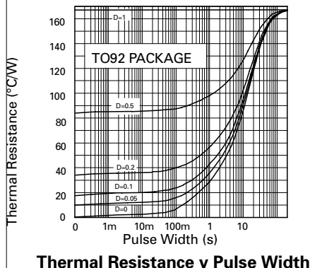
Thermal Resistance v Pulse Width
