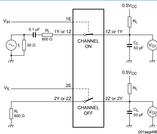
Fig. 16. Test circuit for measuring crosstalk between switches
