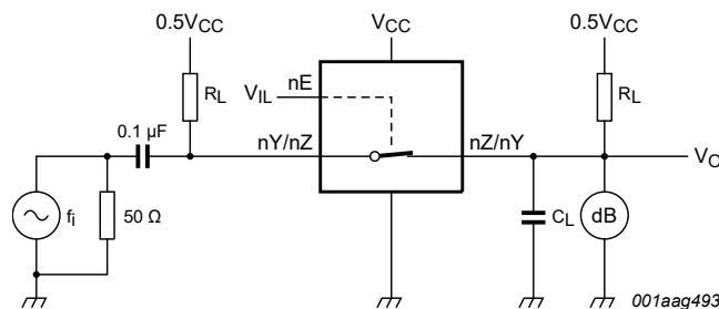
Fig. 14. Test circuit for measuring isolation (OFF-state)
