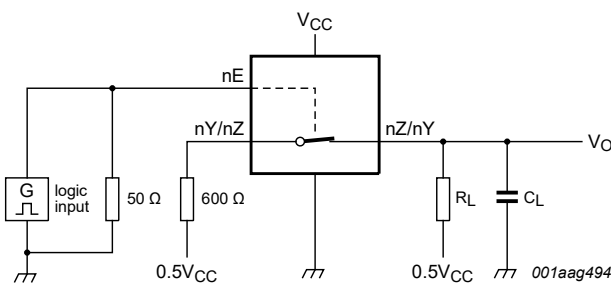
Fig. 15. Test circuit for measuring crosstalk voltage (between digital inputs and switch)
