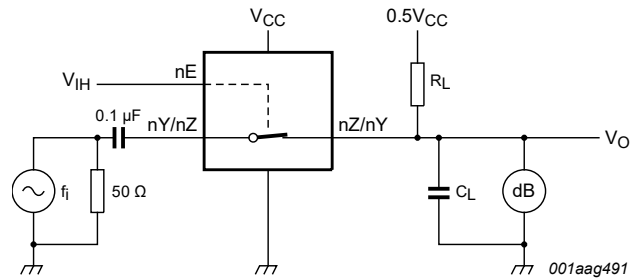
Fig. 13. Test circuit for measuring the frequency response when switch is in ON-state
