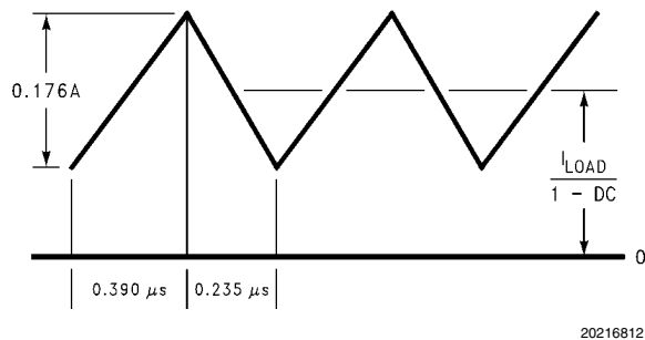
FIGURE 2. 10 \mu\text{H} Inductor Current, 5V–12V Boost
