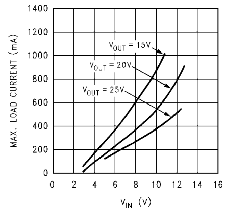
FIGURE 4. Max. Load Current vs V_{\text{IN}}
