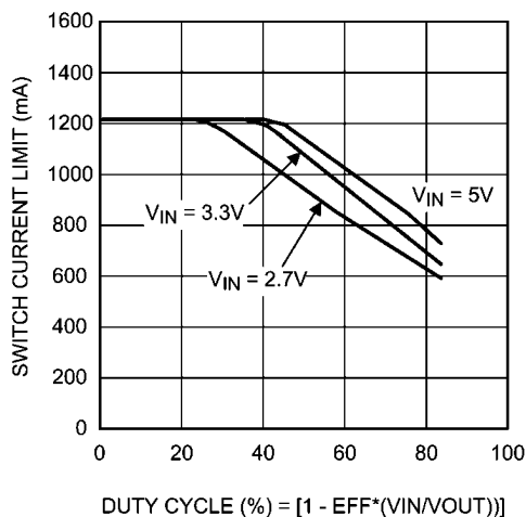
FIGURE 3. Switch Current Limit vs Duty Cycle
