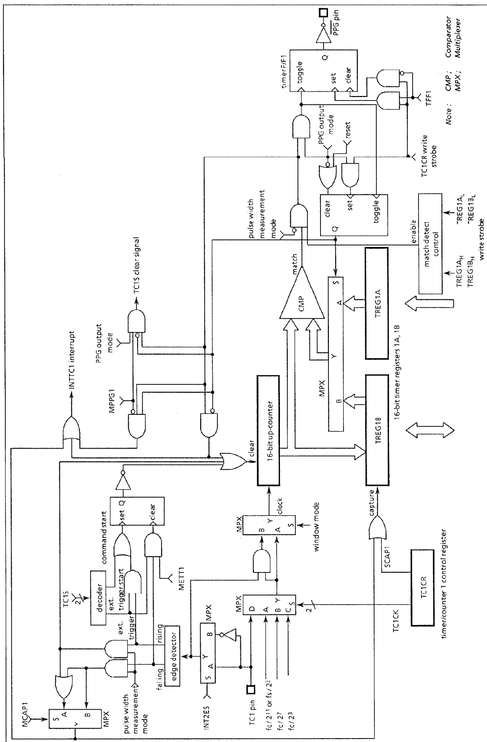
Figure 2-14. Timer/Counter 1
