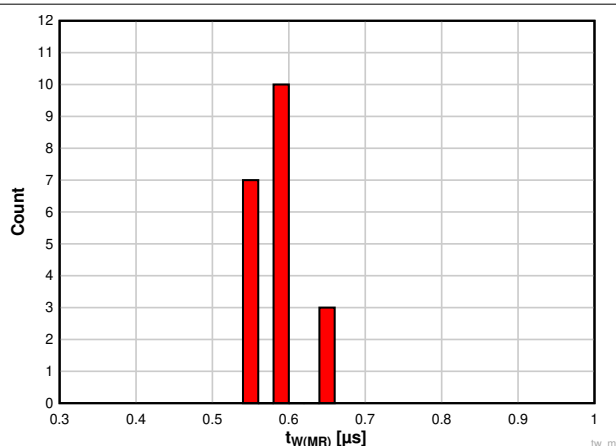
Figure 6-23. Manual Reset Pulse Width Histogram for TPS3823A-33 Devices at 125°C (Unit Count = 20)
