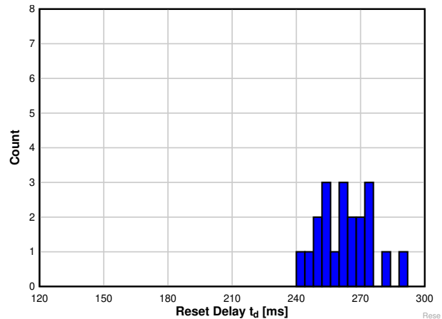
Figure 6-9. Reset Delay Histogram for TPS3823A-33 Devices at -40^{\circ}\text{C} (Unit Count = 20)
