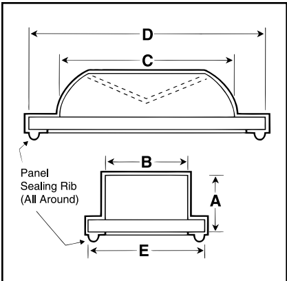
DIMENSIONS FOR REFERENCE ONLY.
