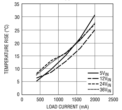
Temperature Rise vs Load Current, V_{OUT} = 2.5V (LGA)
