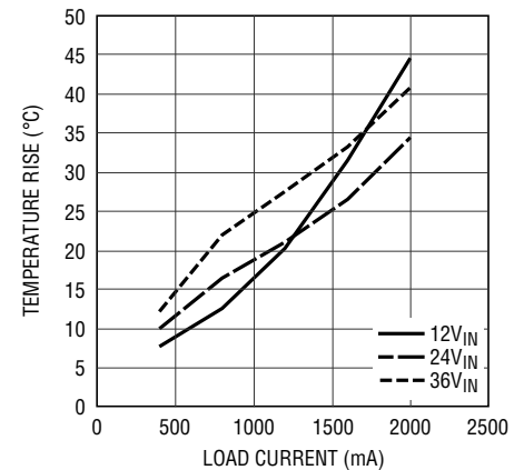
Temperature Rise vs Load Current, V_{OUT} = 8V (LGA)
