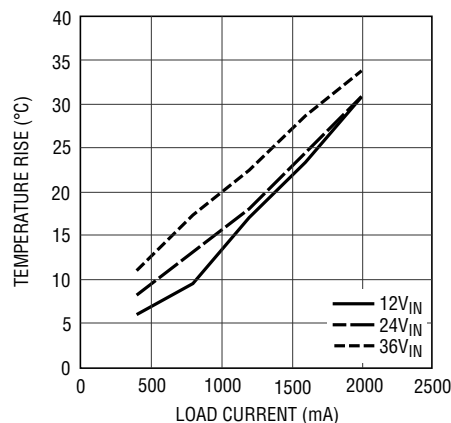
Temperature Rise vs Load Current, V_{OUT} = 5V (LGA)
