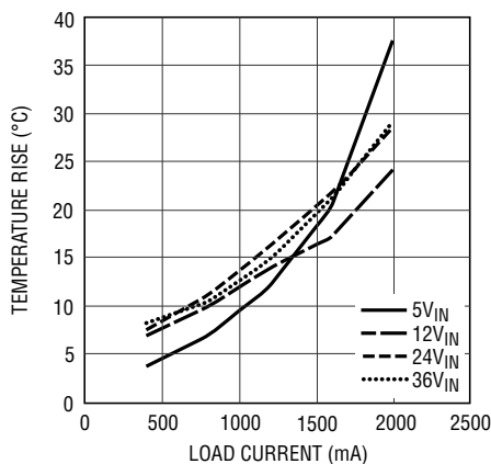
Temperature Rise vs Load Current, V_{OUT} = 3.3V (LGA)
