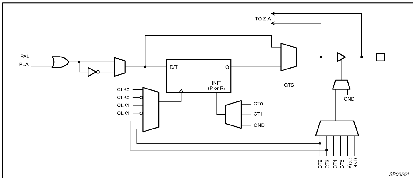
Figure 3. PZ5032C Macrocell Architecture
