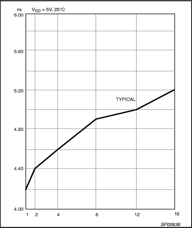
Figure 6. t PD_PAL vs. Outputs switching
