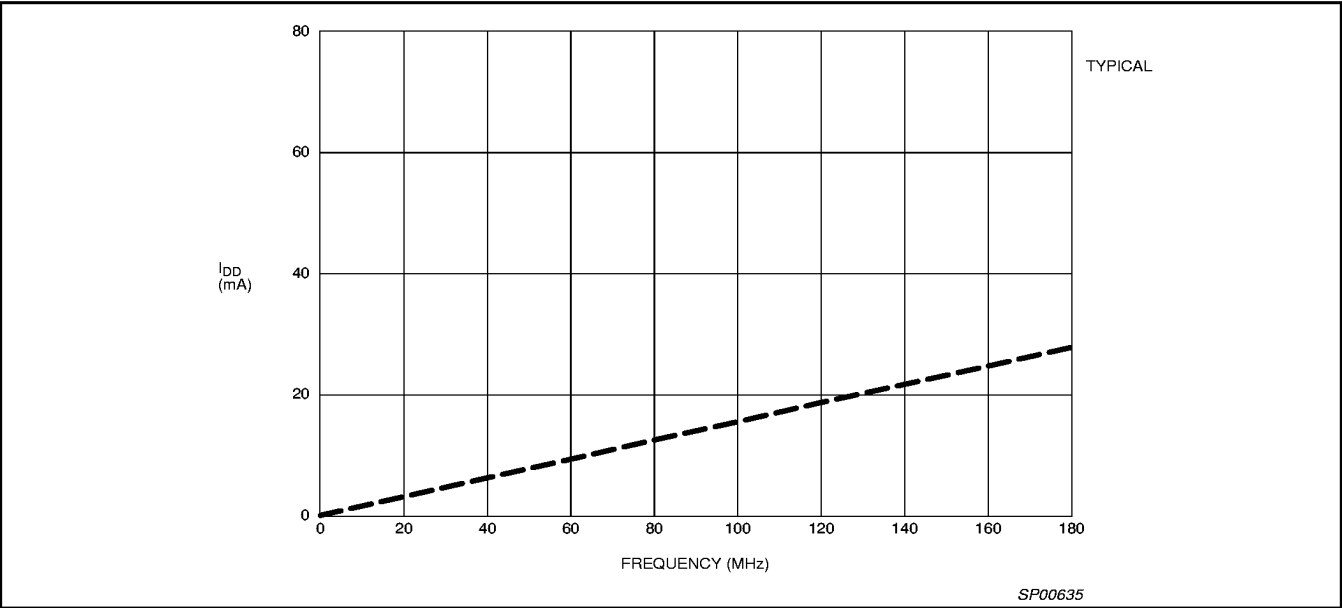
Figure 5. I_{DD} vs. Frequency @ V_{DD} = 5.0\text{V}
