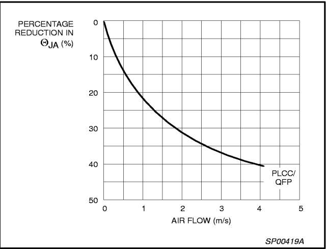
Figure 7. Average Effect of Airflow on \Theta_{JA}
