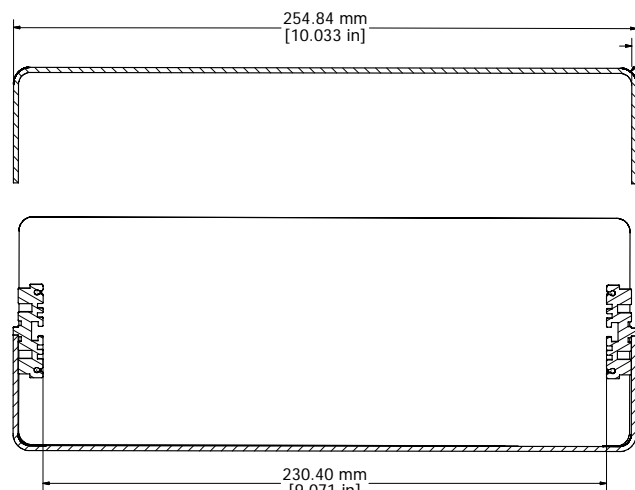
SECTION EE-EE
