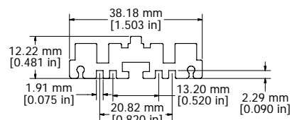
DETAIL GG
