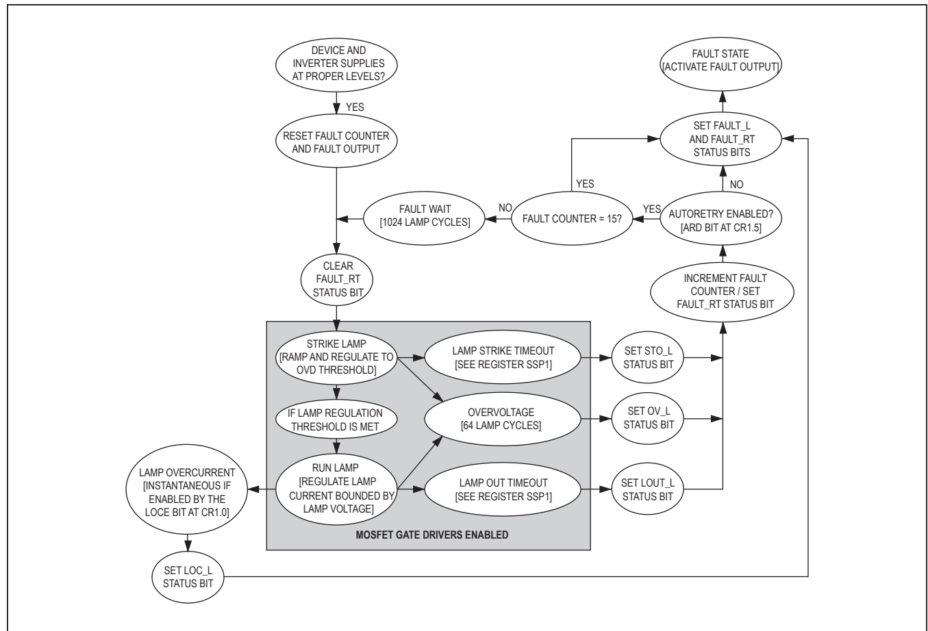
Figure 8. Fault-Handling Flowchart
