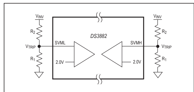
Figure 7. Setting the SVM Threshold Voltage
