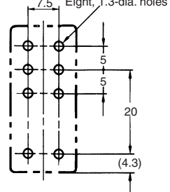
Mounting Holes
