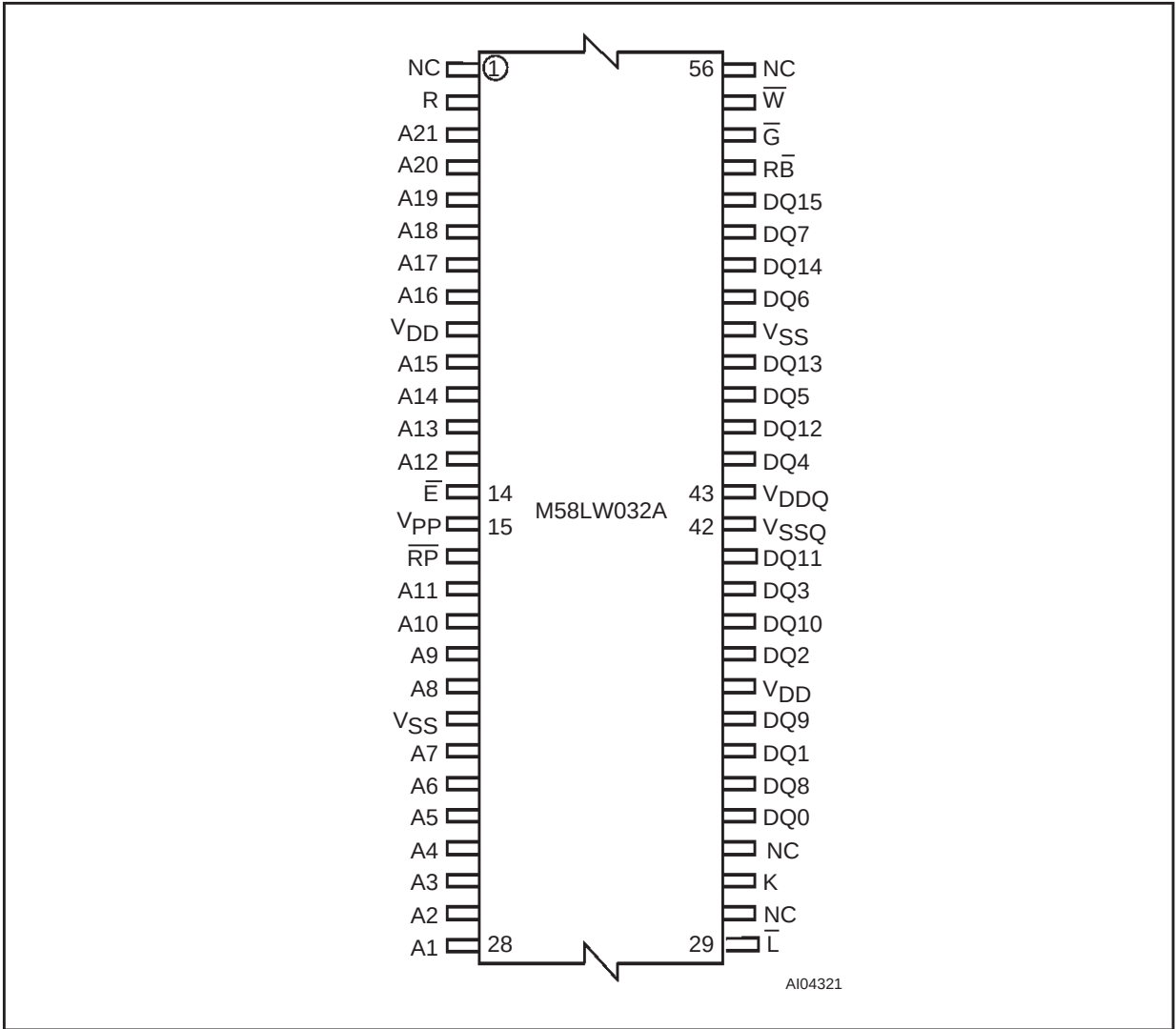
Figure 3. TSOP56 Connections
