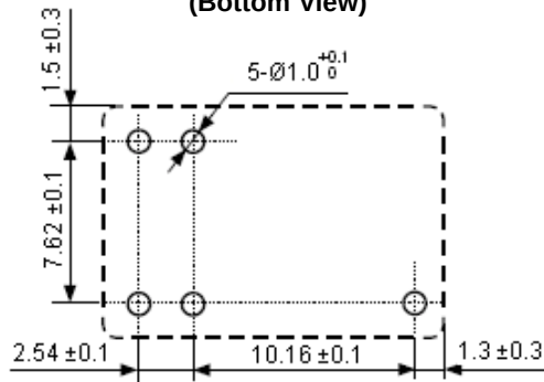
Mounting Hole Layout (Bottom View)
