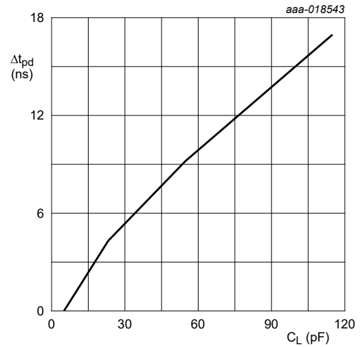
Fig. 12. Additional propagation delay versus load capacitance
