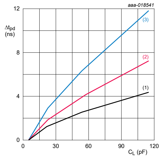
Fig. 8. Additional propagation delay versus load capacitance
