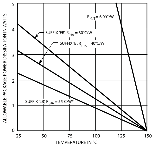
Power Dissipation
