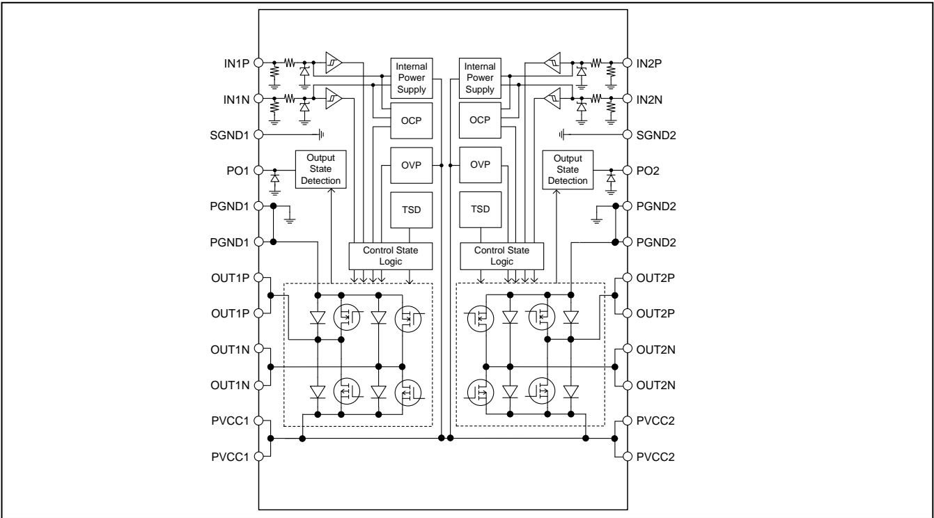
Figure 3. Block Diagram
