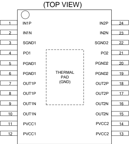
Figure 2. Pin Configuration
