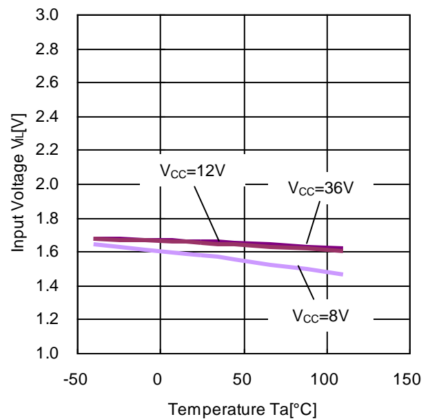
Figure 14. Input Voltage vs Temperature (Input L Voltage V_{IL} , V_{IN}=5.0V \rightarrow 0V )
