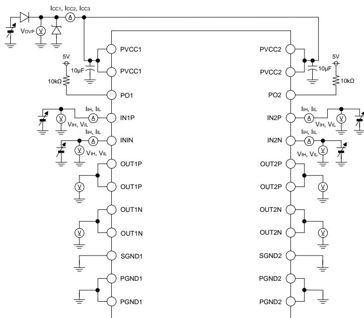
Figure 40. Measurement Circuit 1
