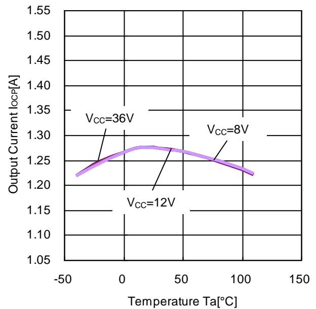
Figure 37. OCP Detect Current vs Temperature (OCP Detect Current Low Side I_{OCP} , I_O = 1.05A \rightarrow 1.55A )
