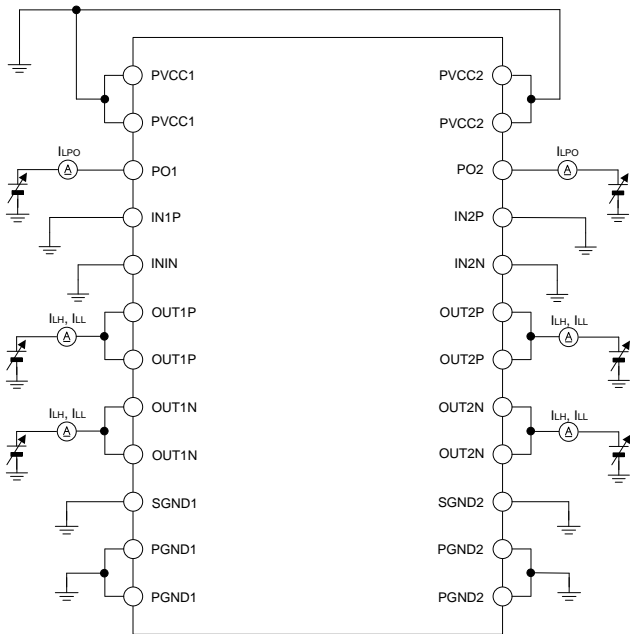
Figure 42. Measurement Circuit 3
