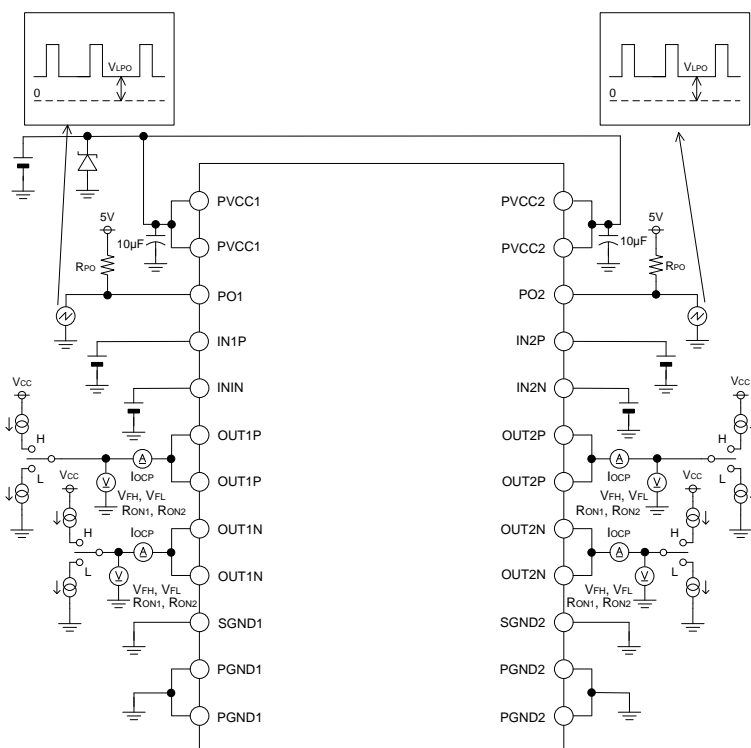
Figure 41. Measurement Circuit 2
