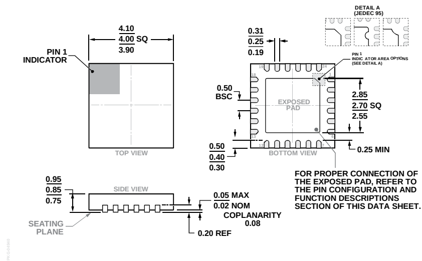
Figure 27. 24-Lead Lead Frame Chip Scale Package [LFCSP] 4 mm × 4 mm Body and 0.85 mm Package Height (HCP-24-3) Dimensions shown in millimeters
