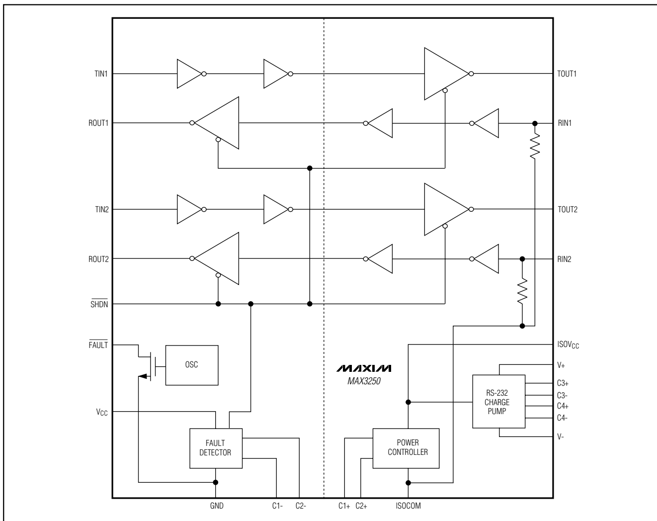
Figure 1. Functional Diagram
