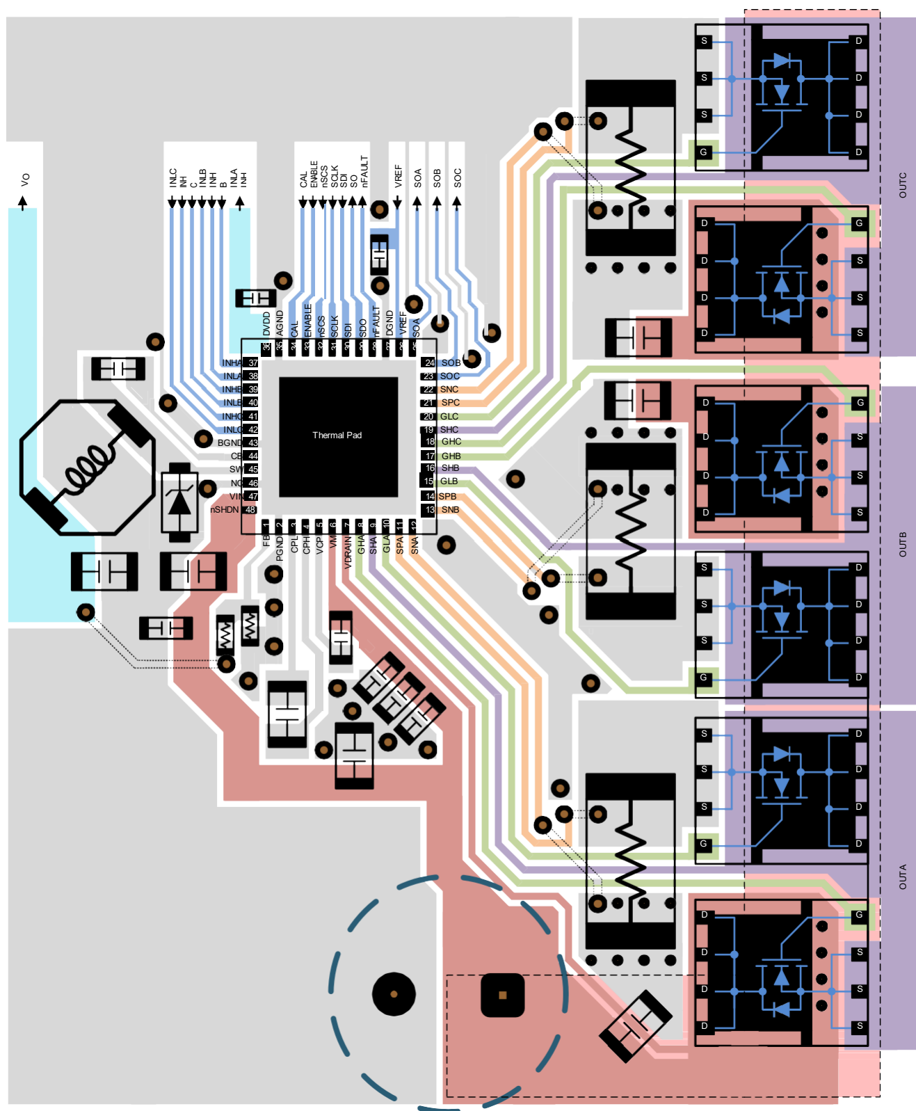
Figure 66. Layout Example
