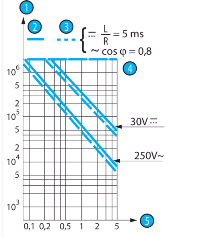
Operating curve for type 83229
