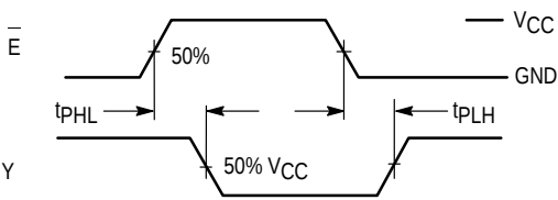
Figure 2. Inverting Switching
