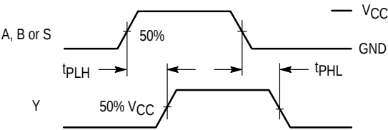
Figure 1. Switching Waveform
