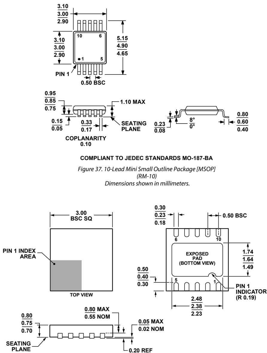
Figure 38. 10-Lead Lead Frame Chip Scale Package [LFCSP]
