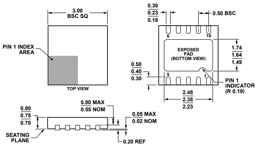
Figure 38. 10-Lead Lead Frame Chip Scale Package [LFCSP]
