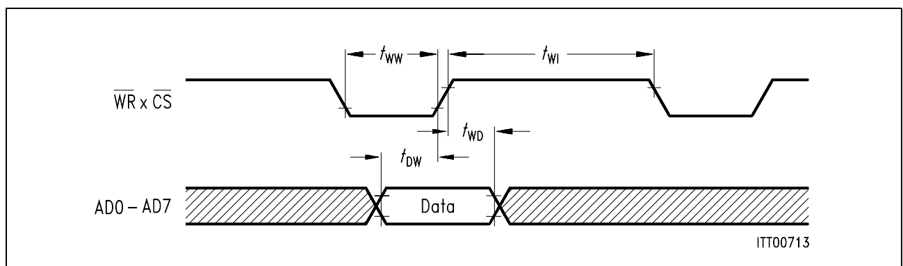
Figure 96 Microprocessor Write Cycle
