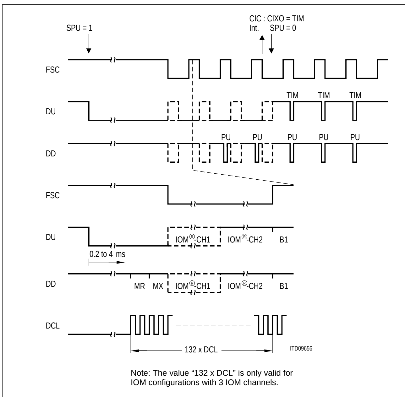
Figure 78 Activation of the IOM-2 interface
