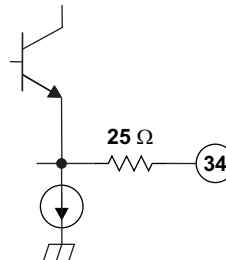
Figure 10. MIXOUT1 and MIXOUT2
